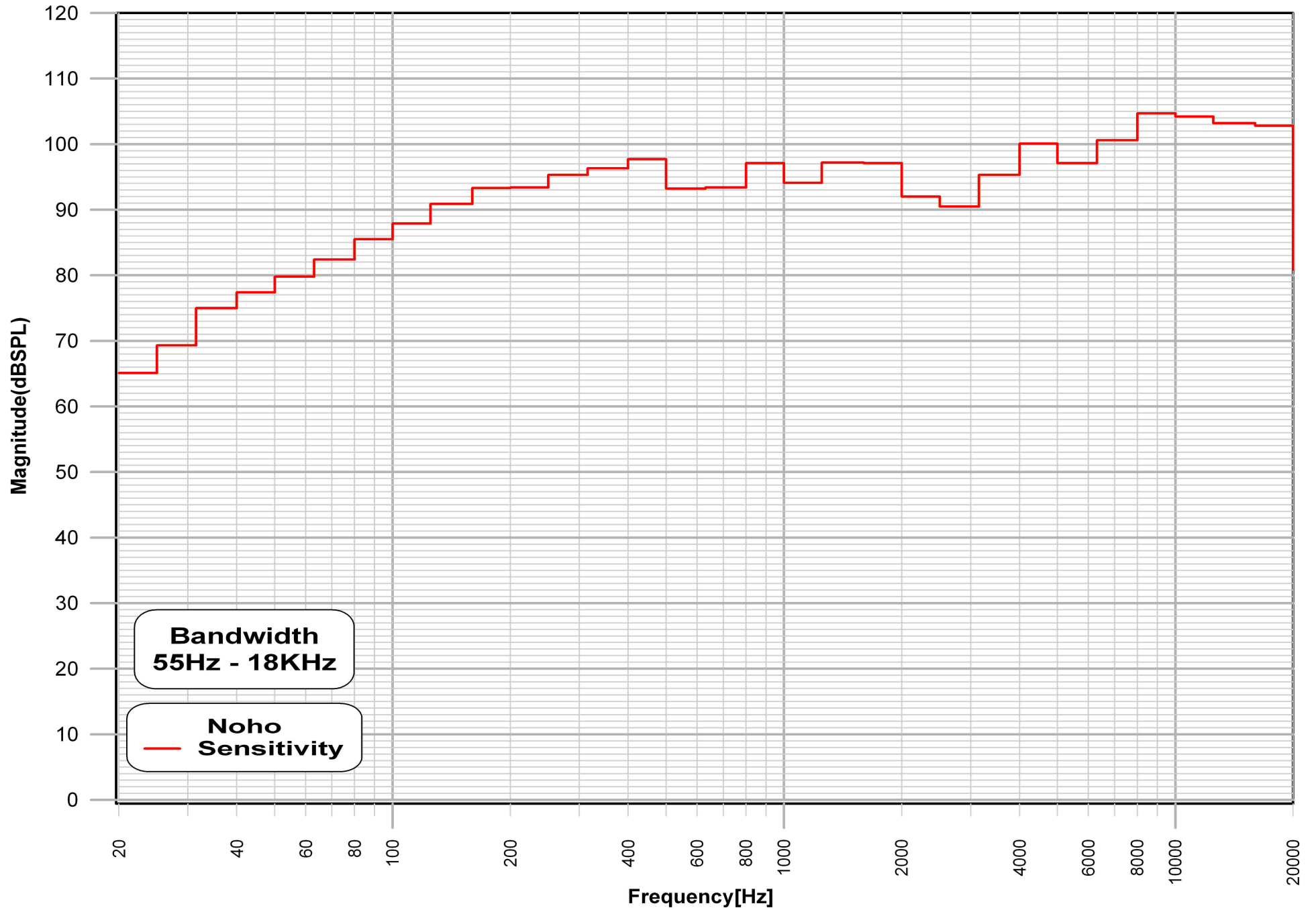
1/3 Octave Sensitivity Plot
